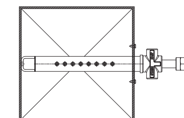
Vertical duct (plan view)
